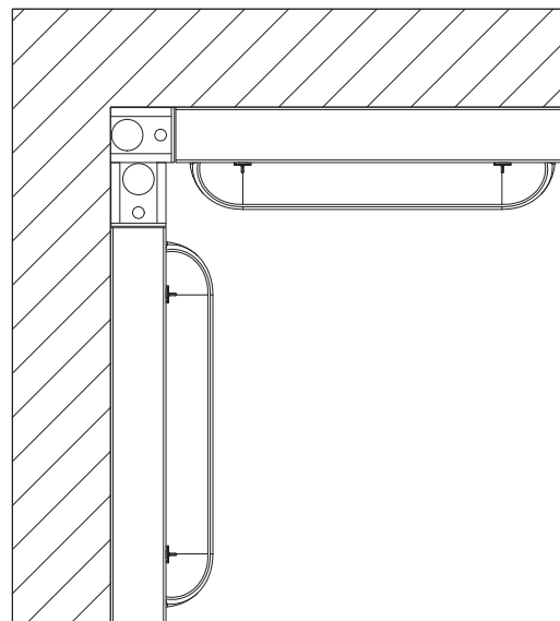
Internal corner - option 4
