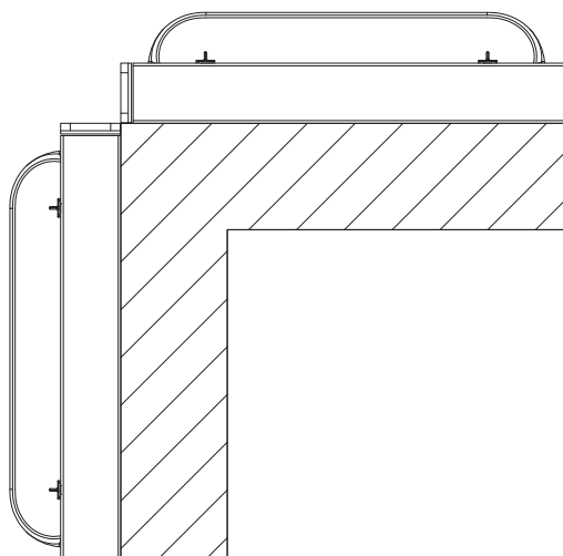
External corner - option 1
