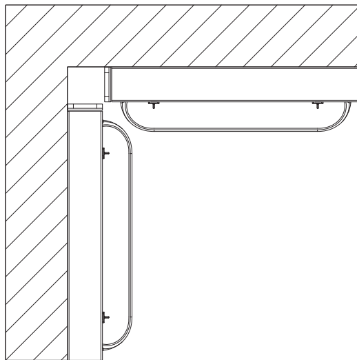
Internal corner - option 4
