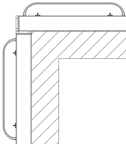
External corner - option 2
