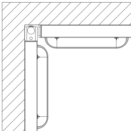
Internal corner - option 3
