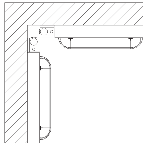
Internal corner - option 5
