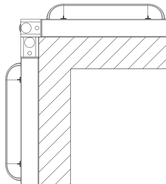
External corner - option 6
