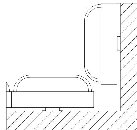
Internal corner
