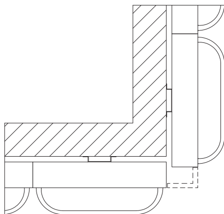
External corner - option 1
