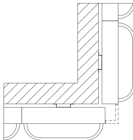
External corner - option 2
