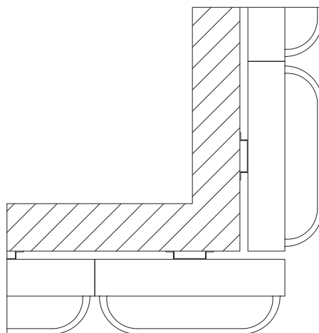
External corner - option 4
